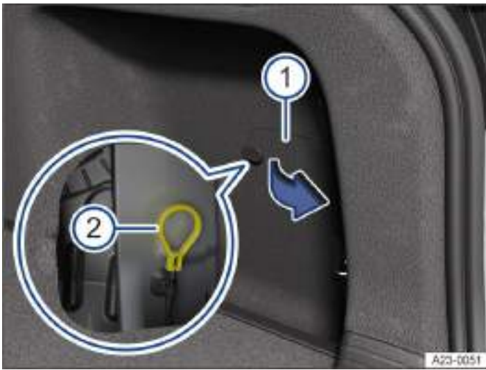
Fig. 2 In the lower right-hand side of the luggage compartment trim: manual release of the charging connector.
