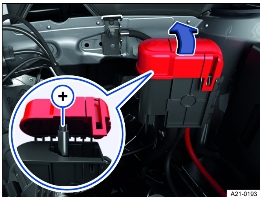
Fig. 161 Under a cover in the engine compartment: Positive jump-start point.
