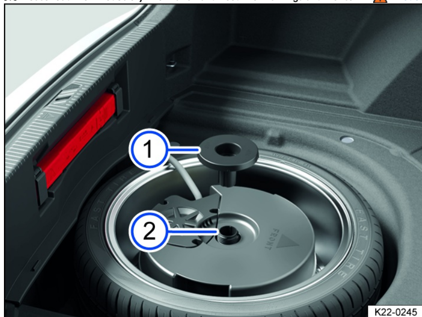
Fig. 188 Removing the subwoofer.
