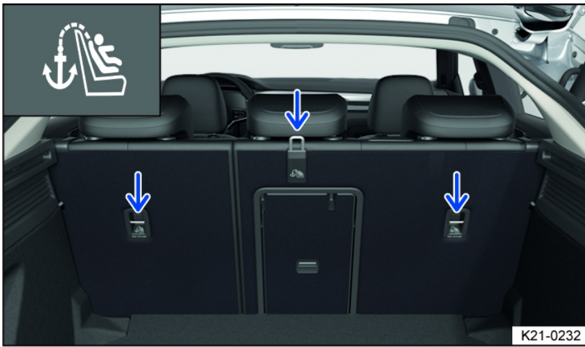
Fig. 38 On the rear side of the rear bench seat: Top tether anchorages for the top tether safety belt.
