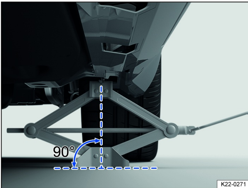
Fig. 194 Jack is positioned on the left side of the vehicle at the rear.
