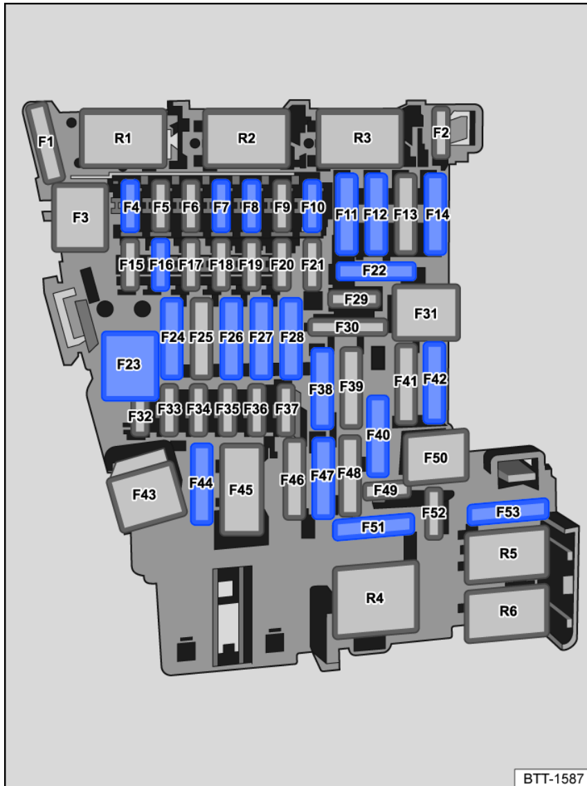
Fig. 157 Fuse assignment in the instrument panel.
