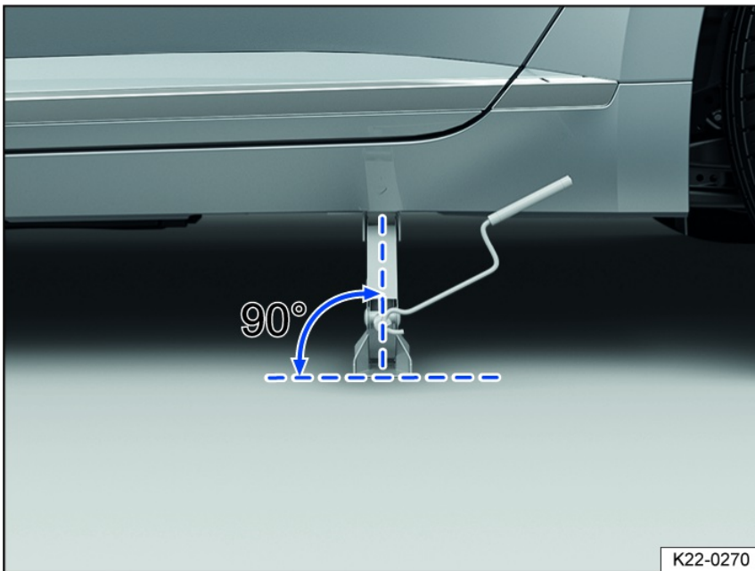
Fig. 193 Correct jack setup.
