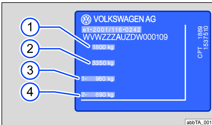
Fig. 207 Identification label (general example): version 2.
