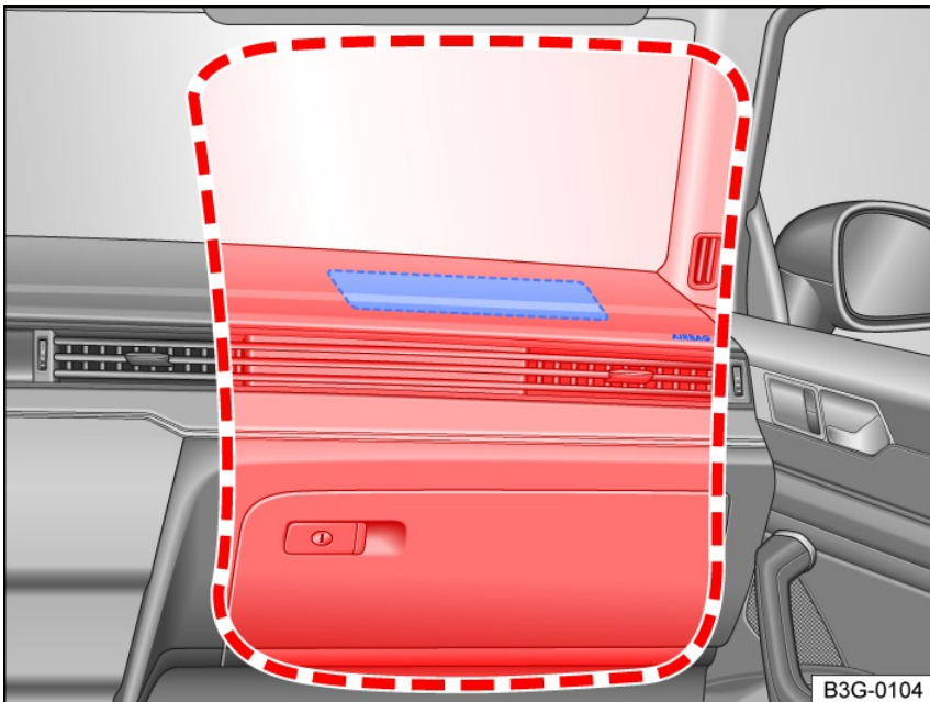
Fig. 27 Installation location and deployment zone of the front passenger's front airbag.
