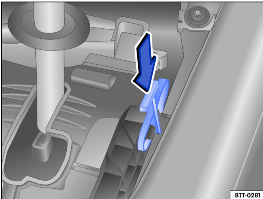
Fig. 103 Manually release the Automatic Shift Lock (ASL) (variant 2).
