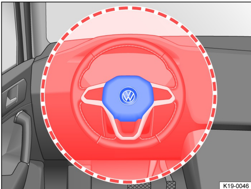
Fig. 26 Installation location and deployment zone of the driver's front airbag.
