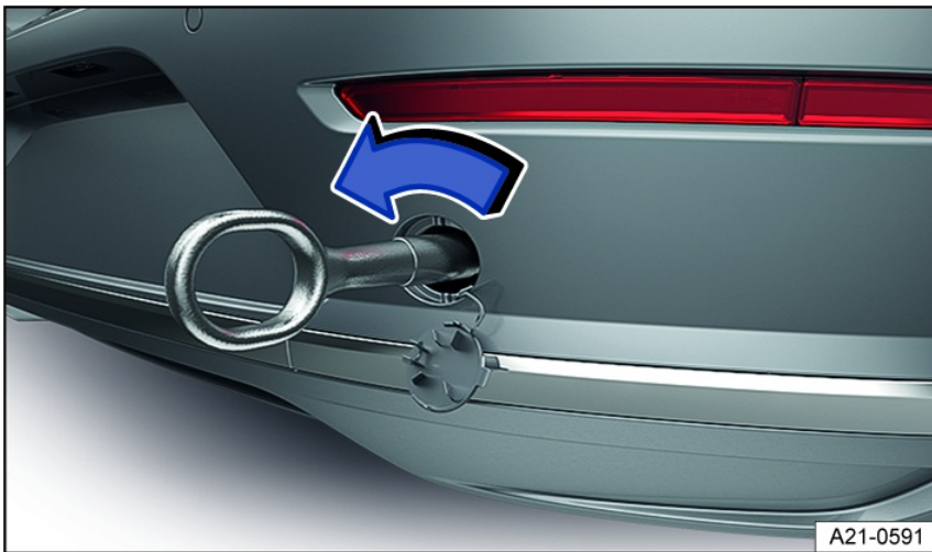
Fig. 167 In the right rear bumper: Screw in towing eye.
