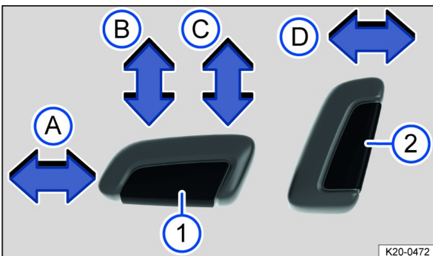
Fig. 69 Switch on the driver seat: Adjusting the front seat forward/back, the height and angle of the seat surface, and the front seat backrest.
