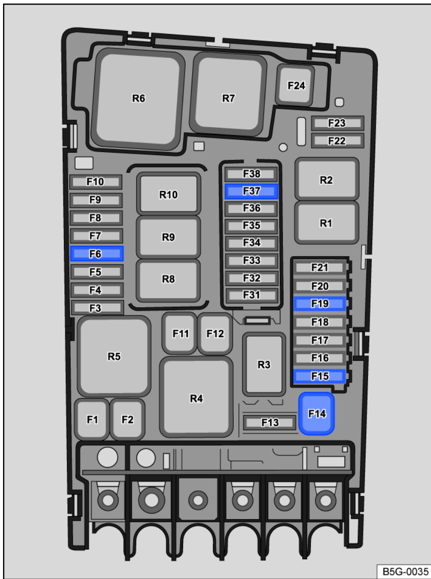
Fig. 154 Fuse locations in the engine compartment.
