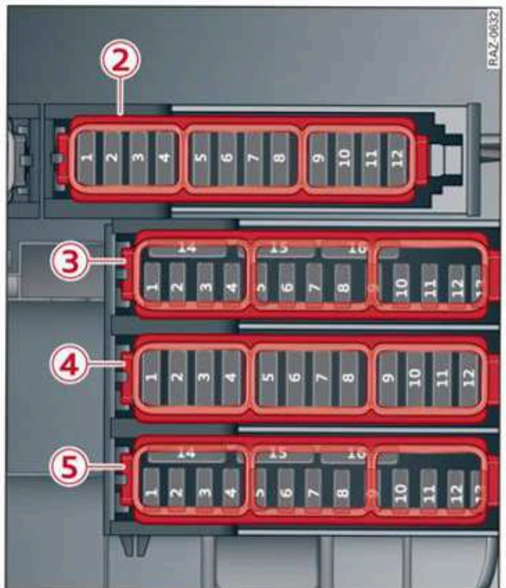
Fig. 186 Front passenger footwell: fuse panel with plastic clip
