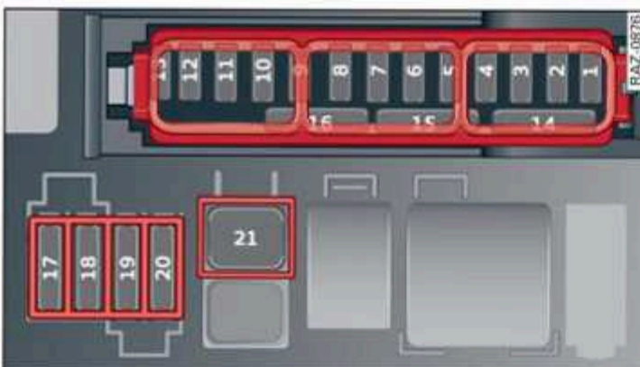
Fig. 184 Right side of the front compartment: fuse panel with plastic clip
