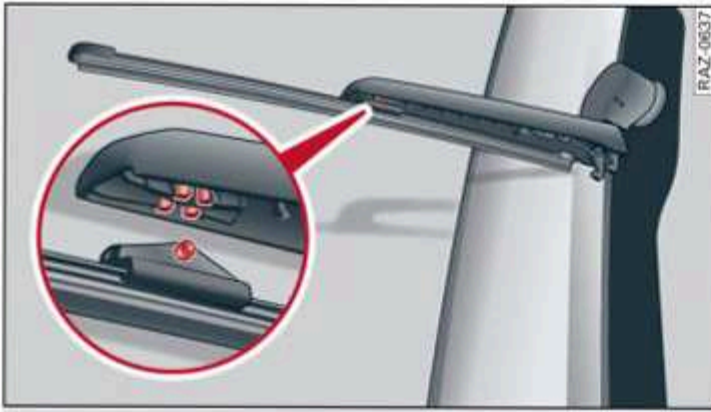
Fig. 48 Rear window wiper: installing the wiper blade
