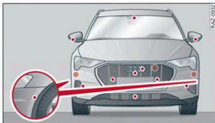
Fig. 98 Front area: sensors and cameras
