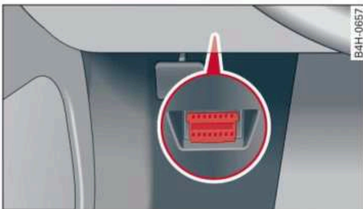
Fig. 188 Driver's side footwell: connection port for the On Board Diagnostic System (OBD)
