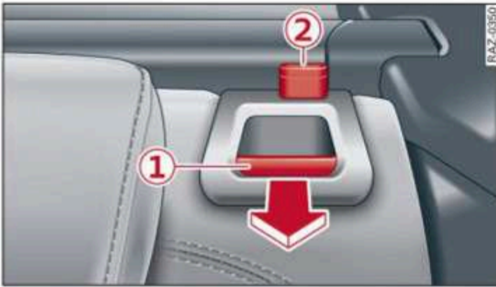
Fig. 75 Outer backrest: release lever and latching indicator with red marking
