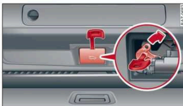
Fig. 33 Inner luggage compartment lid: access to the emergency release
