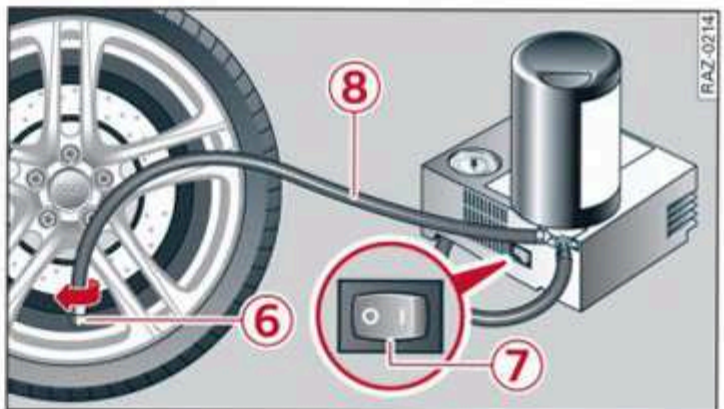
Fig. 172 Tire mobility kit connection
