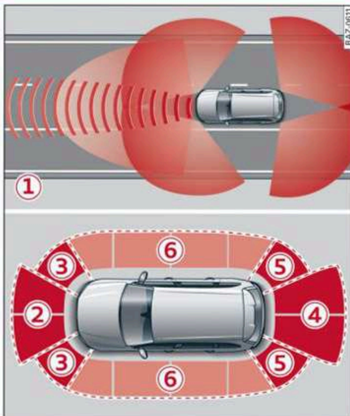
Fig. 96 Sensor coverage area
