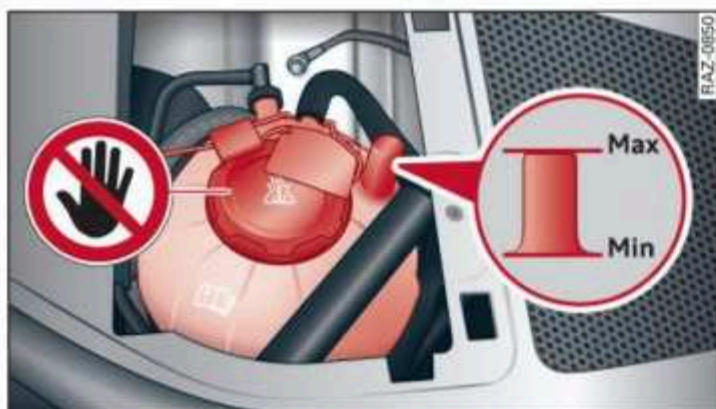
Fig. 162 Front compartment: coolant expansion tank
