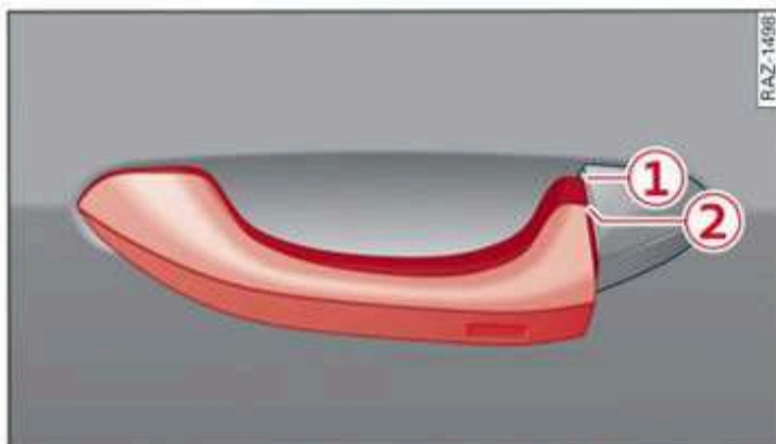
Fig. 22 Door handle: ① standard operation, ② emergency operation
