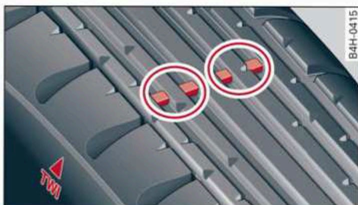
Fig. 166 Tire profile: treadwear indicator
