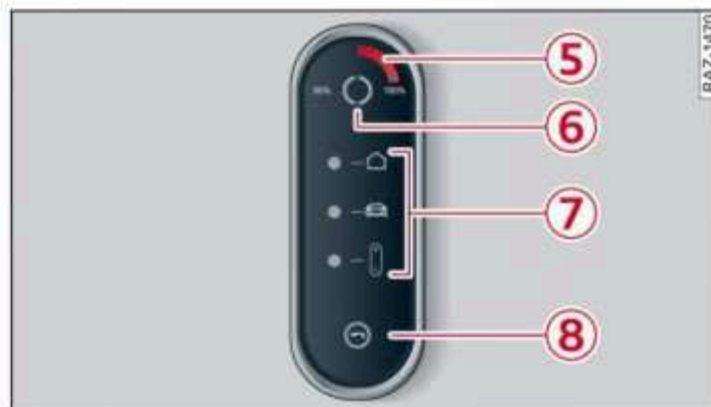
Fig. 92 Audi e-tron compact charging system: control unit
