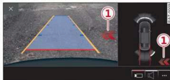
Fig. 133 Upper display: rear cross-traffic assist display
