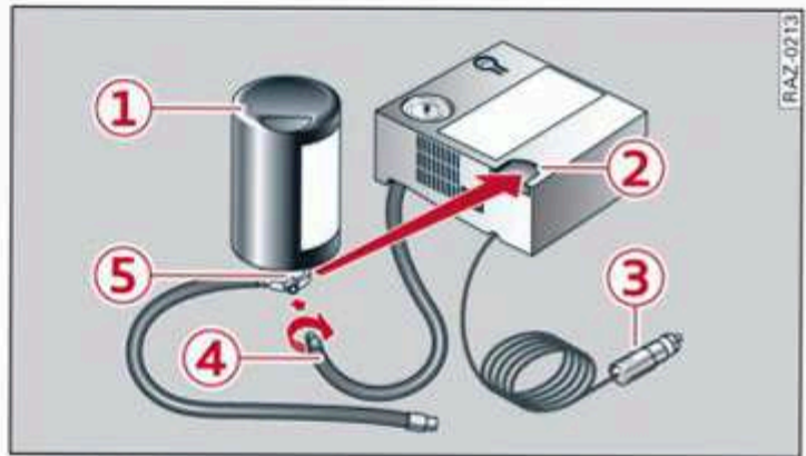
Fig. 171 Components of the tire mobility kit
