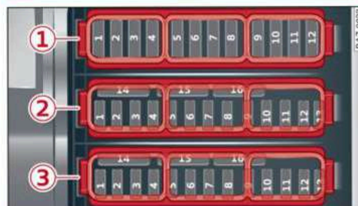
Fig. 187 Left side of the luggage compartment: fuse panel with plastic clip
