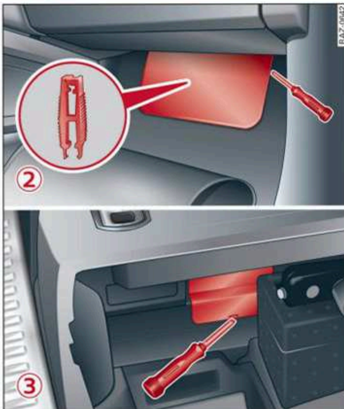
Fig. 183 Front passenger footwell: cover and clip ②, left side of the luggage compartment: cover ③
