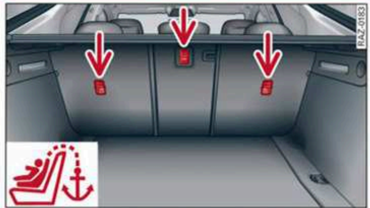
Fig. 65 Rear backrest: top tether anchors to secure a child safety seat with an upper belt
