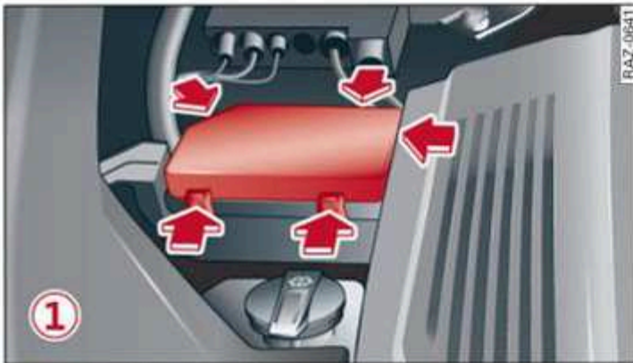
Fig. 182 Right side of the front compartment: fuse panel cover ①
