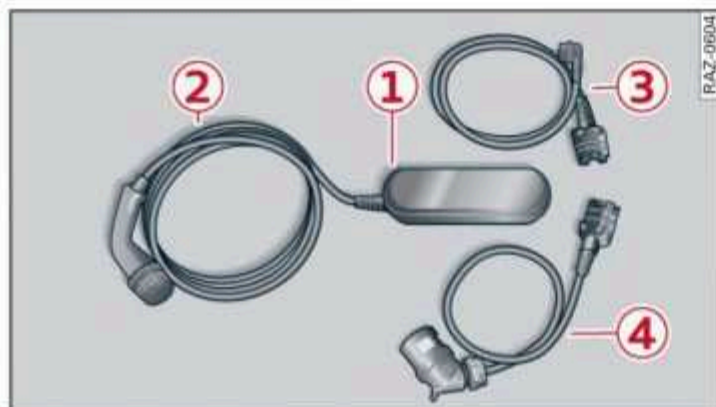
Fig. 91 Audi e-tron compact charging system: components (example)
